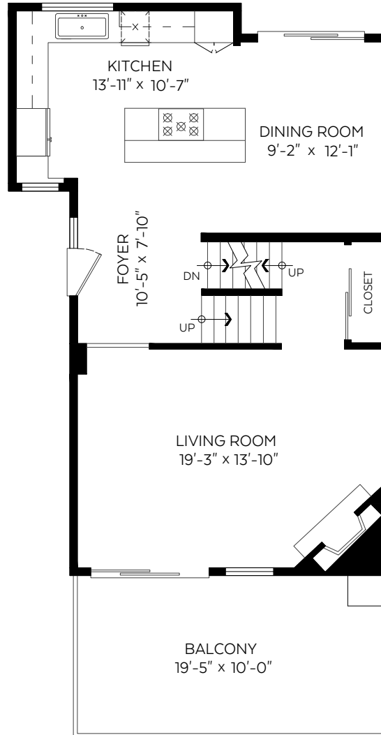
Main Floor Plan Floor Area: 758 sq.ft.
