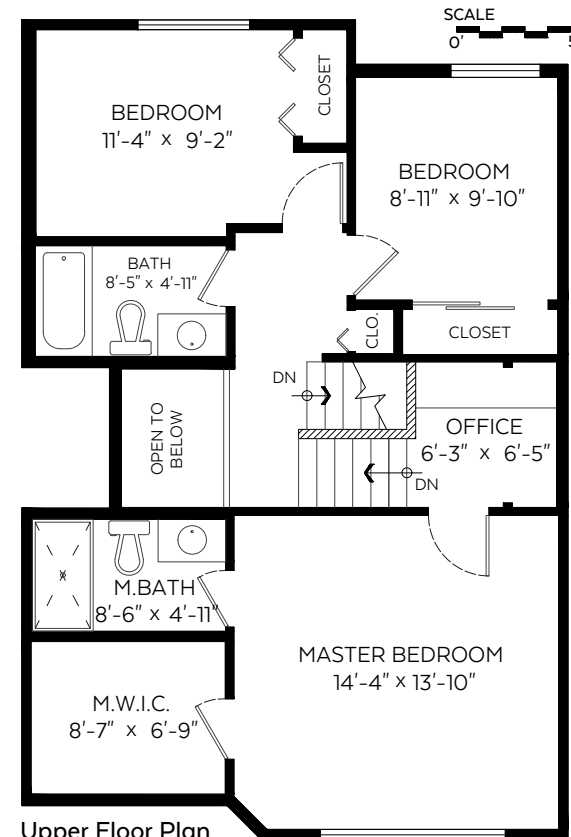
Upper Floor Plan Floor Area: 782 sq.ft.
