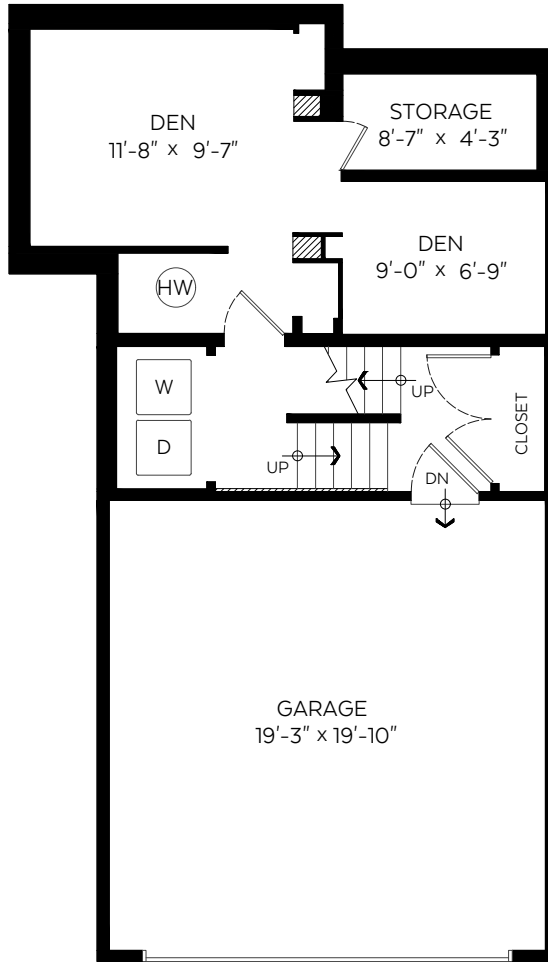
Lower Floor Plan Floor Area: 469 sq.ft.
